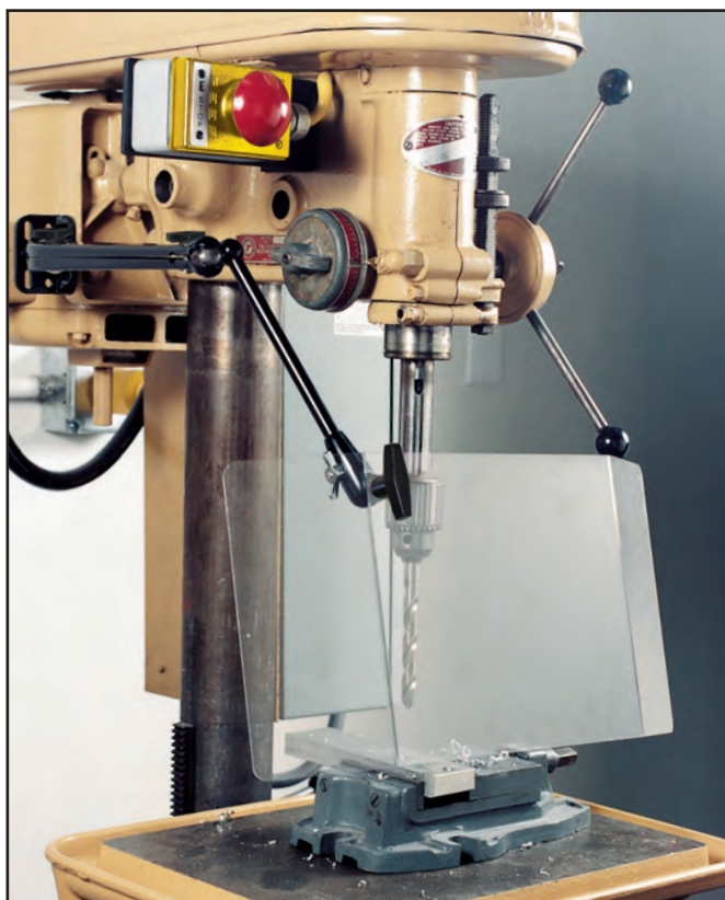
Universal ball & socket shield shown on a drill press.
