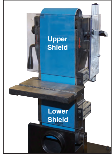
Belt sander shield assembly.
