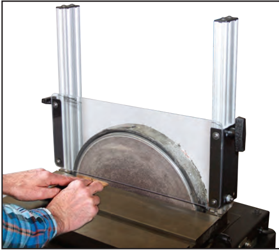
Disc sander shield assembly.
