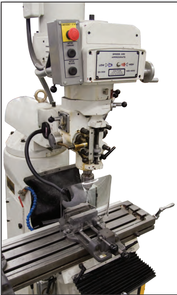
Flexible spring-steel arm shield on milling machine.
